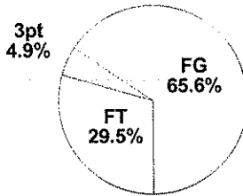
Scoring Distribution
