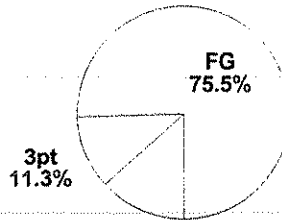
Scoring Distribution
