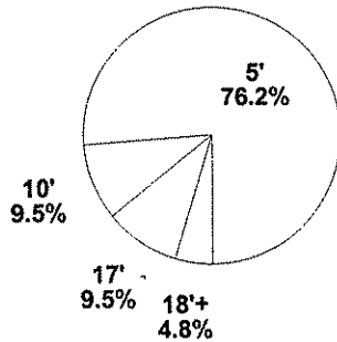
Scoring Range
