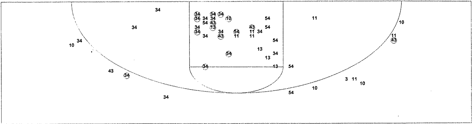
Scoring Distribution
